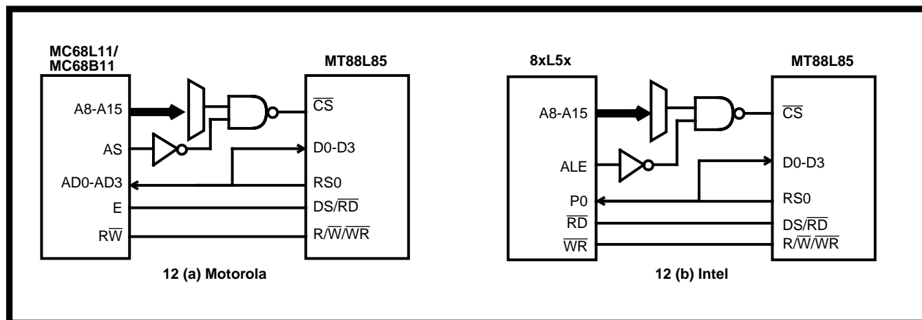
Figure 12 a) & b) - MT88L85 Interface Connections for Various Intel and Motorola Micros
